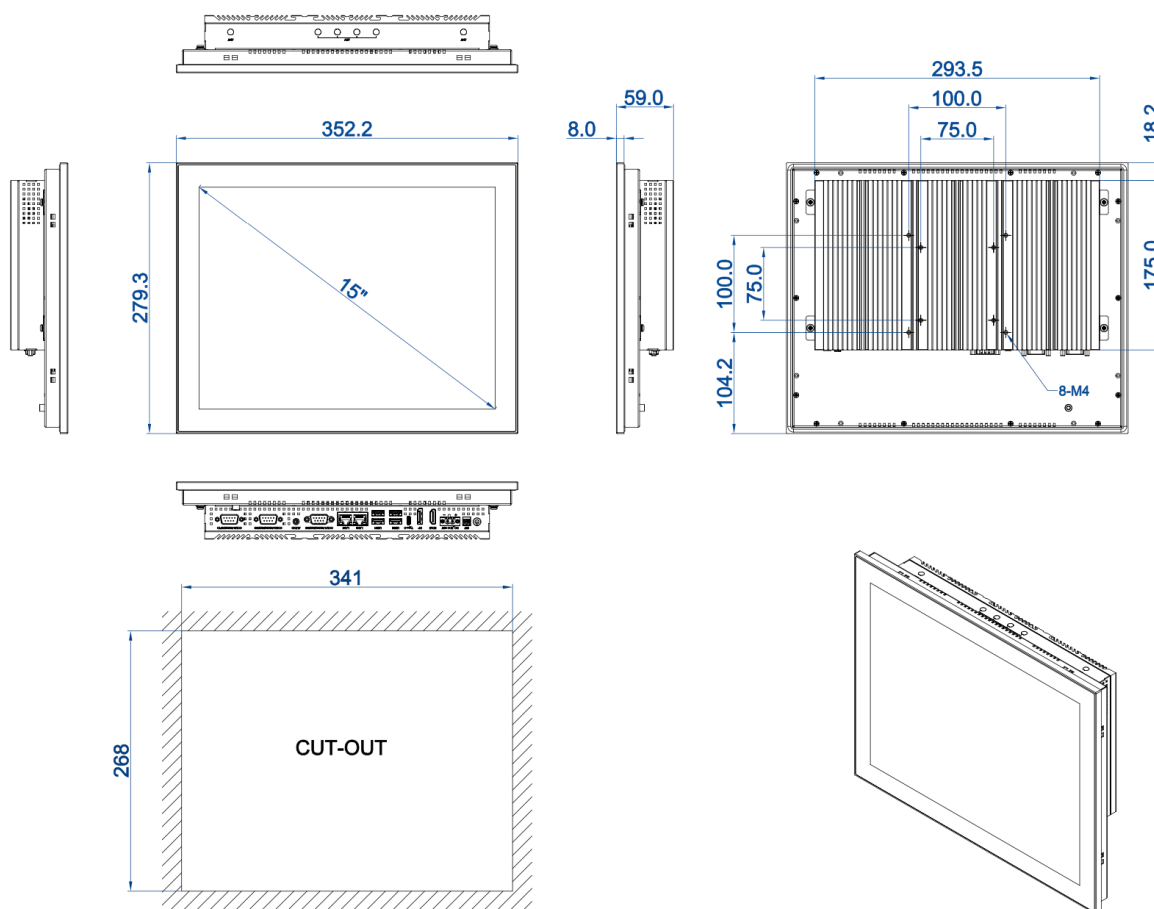
DIMENSIONAL DRAWING:TPC-DCT150D
