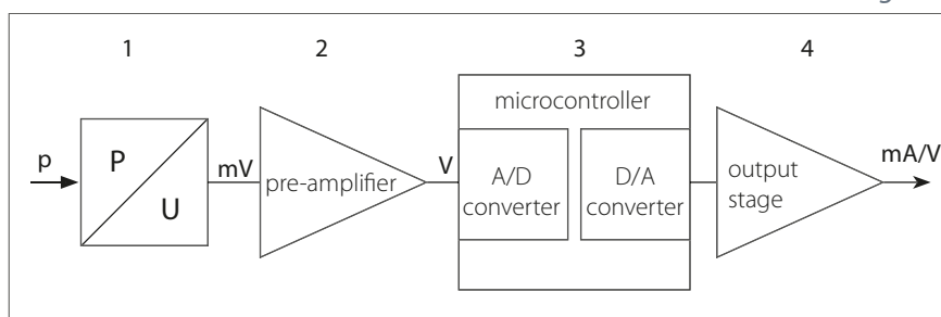
Block diagram:
